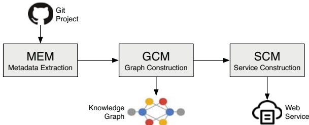
Fig. 1. GitGraph Overview.
