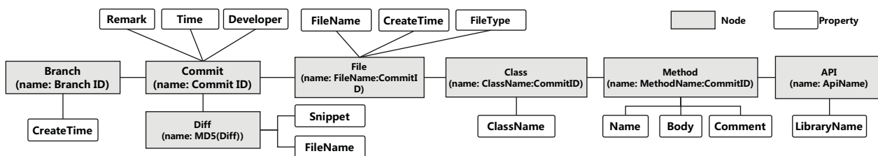
Fig. 2. The Schema of GitGraph's Graph Database
